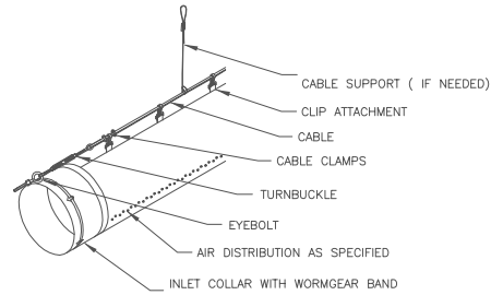
SUSPENSION DETAIL 1 ROW CABLE SUSPENSION AT 12 O'CLOCK
