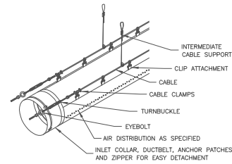
SUSPENSION DETAIL 2 ROW CABLE SUSPENSION AT 10&2 O'CLOCK
